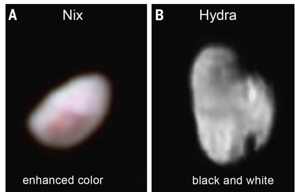
Fig. 7. LORRI and Ralph surface imaging of Nix and Hydra. (A) Nix Ralph color composite image at 3.14 km/pixel with a solar phase angle of 15^\circ , created by combining images taken through three filters (near-IR, 780 to 975 nm; red, 540 to 700 nm; blue, 400 to 550 nm) that were respectively loaded in the red, green, and blue planes of the color composite. (B) LORRI panchromatic (350 to 850 nm) image of Hydra at 1.13 km/pixel, solar phase angle 34^\circ .
